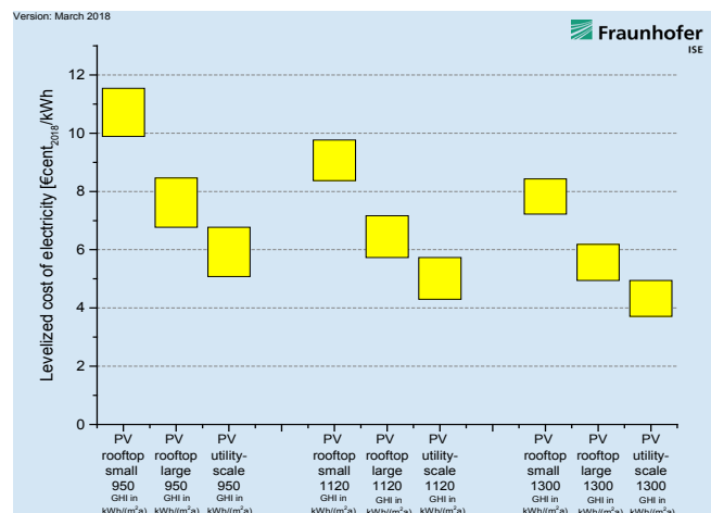
Figure 6: LCOE of PV plants in Germany based on system type and solar irradiance (GHI in kWh/(m 2 a)) in 2018.
