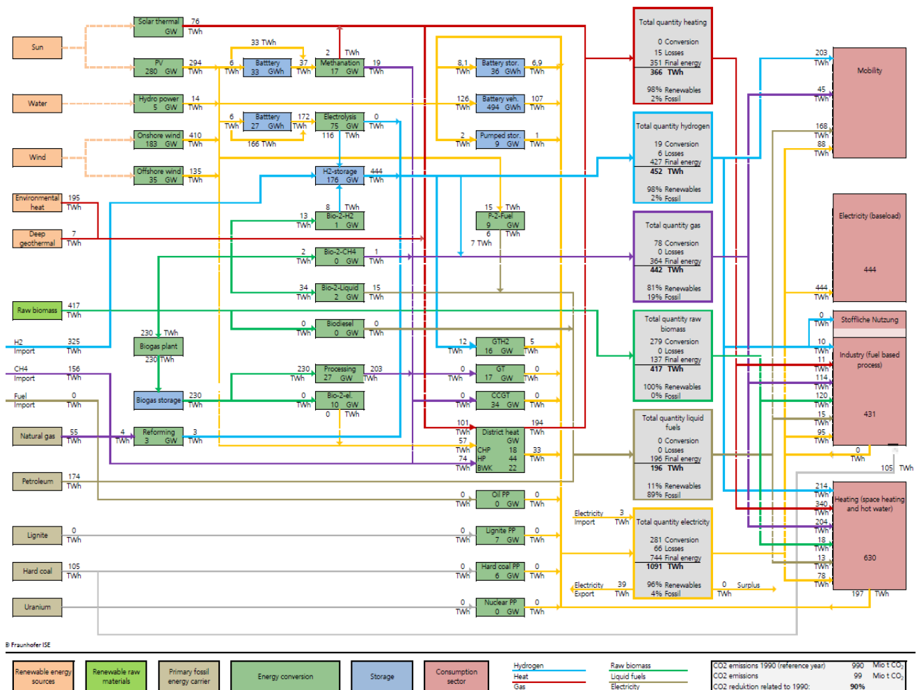
Figure 23: Scheme of the energy system depicted in the simulation model REMod with exemplary values of a scenario in 2050. The diagram shows all conversion paths from fossil primary energy or renewable energies to the respective consumption sectors
