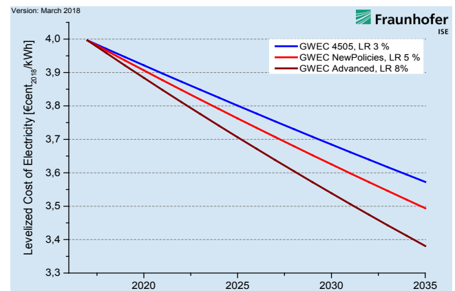
Figure 18: Sensitivity analysis for the LCOE forecast of Onshore-wind power, investment costs in 2018 = 1500 EUR/kWh, FLH are increasing from 3200 h/a in 2018 to 3500 h/a in the year 2035.
