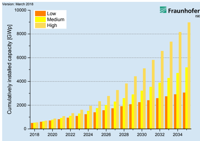
Figure 5: Market development scenarios of cumulatively installed power plant capacity [GW] for PV 2018-2035, own scenarios.
