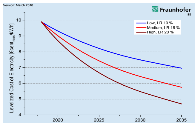
Figure 17: Sensitivity analysis for the LCOE forecast of small PV plants, investment costs in 2018 = 1200 EUR/kWh, GHI=950 kWh/(m 2 a).
