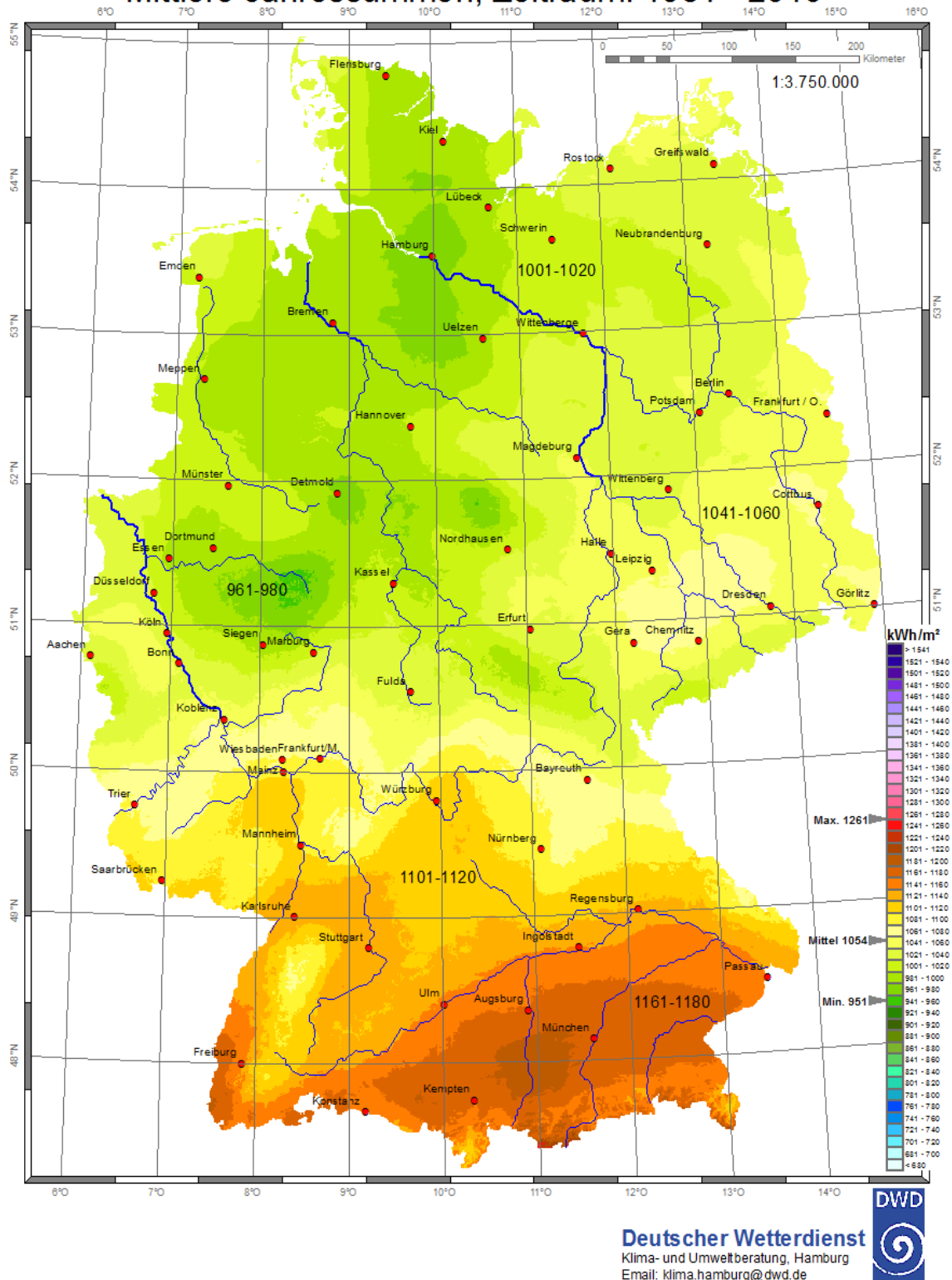
Figure 25: Average annual sum of global irradiance [kWh/m 2 ] in Germany from 1981-2010 (DWD 2013)
