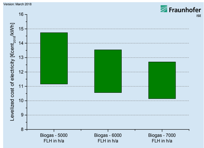
Figure 11: LCOE of biogas power plants at different FLH in 2018.
