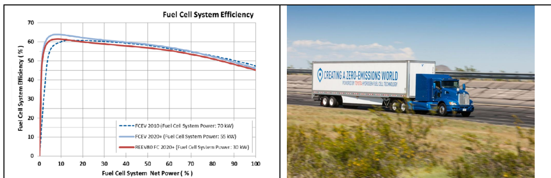
Figuur 2.10 brandstofcel efficiency range extender en full FC
